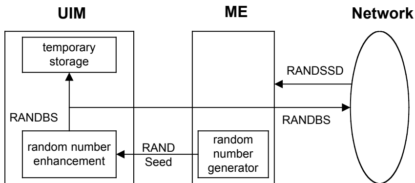
Figure 2. Base Station Challenge Function
